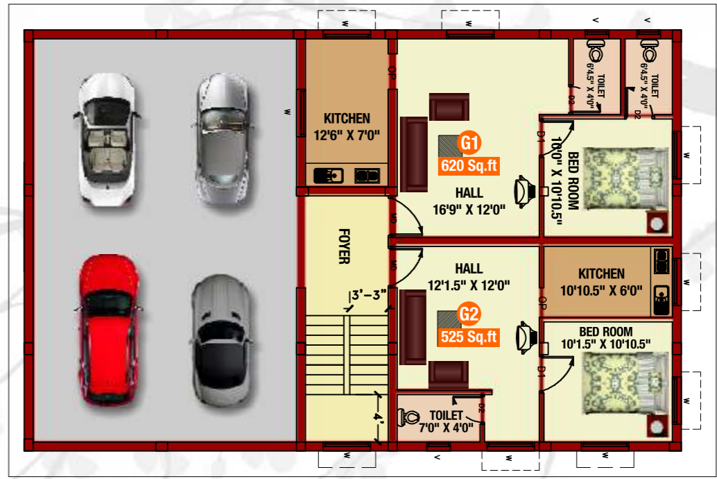
Block C & D Typical Floor Plan
